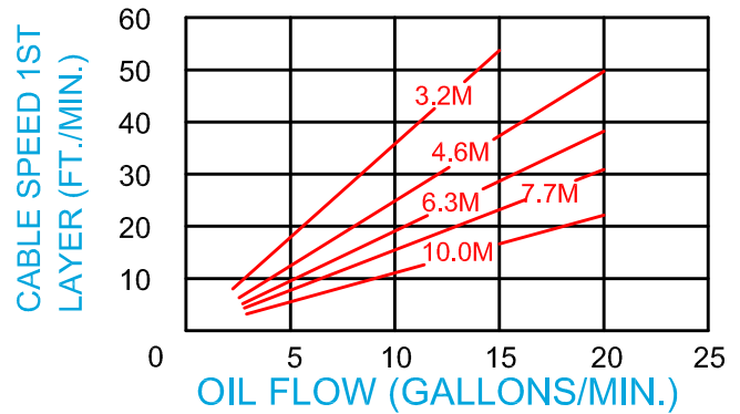
20:1 RATIO (standard)
