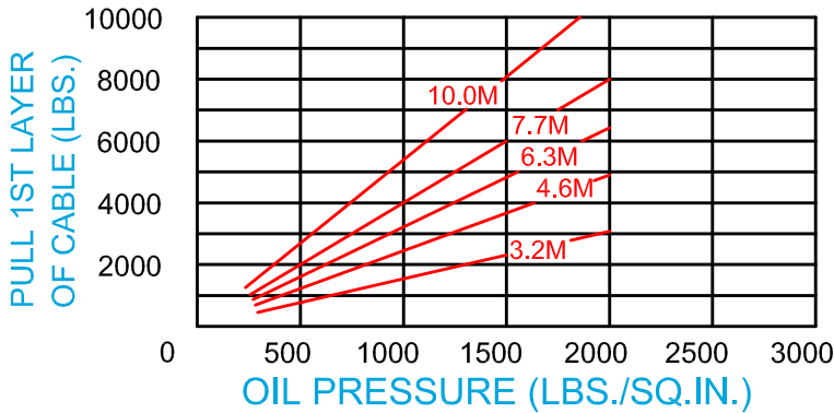
27:1 RATIO (optional)
