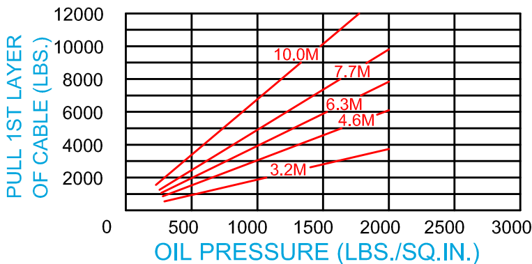
40:1 RATIO (optional)
